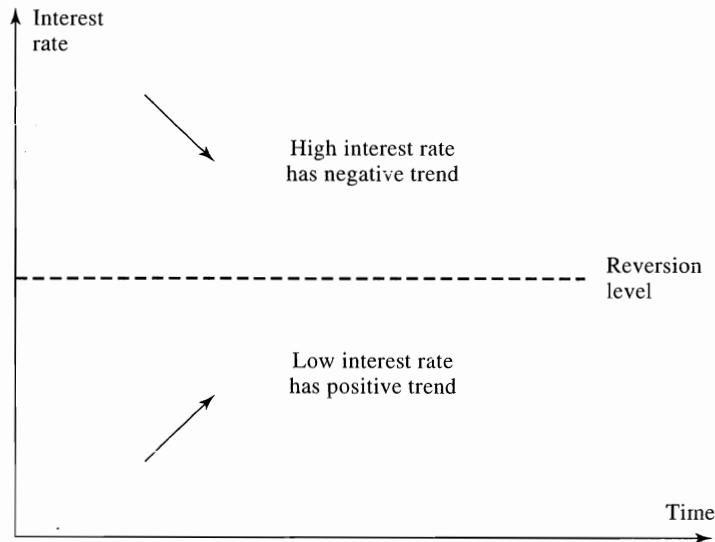
Figure 30.1 Mean reversion.
