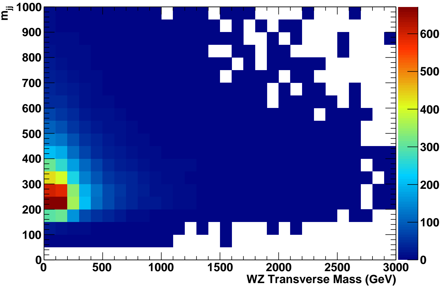
m_{jj} vs. WZ Transverse Mass Max QCD (Standard Model)
