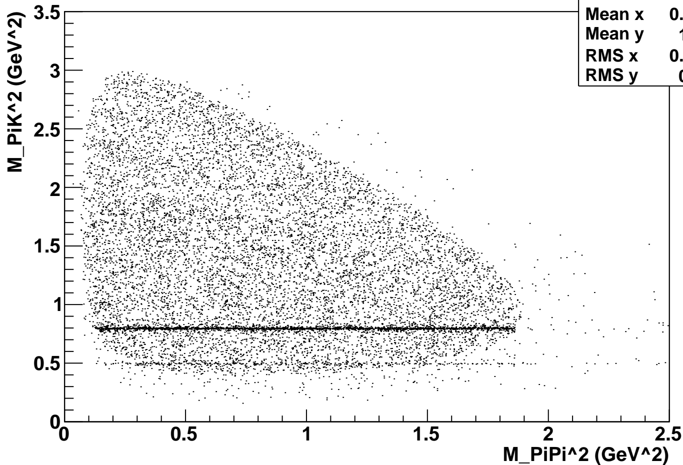
Dalitz Plot D \rightarrow K + 2Pi (GeV 2 )
