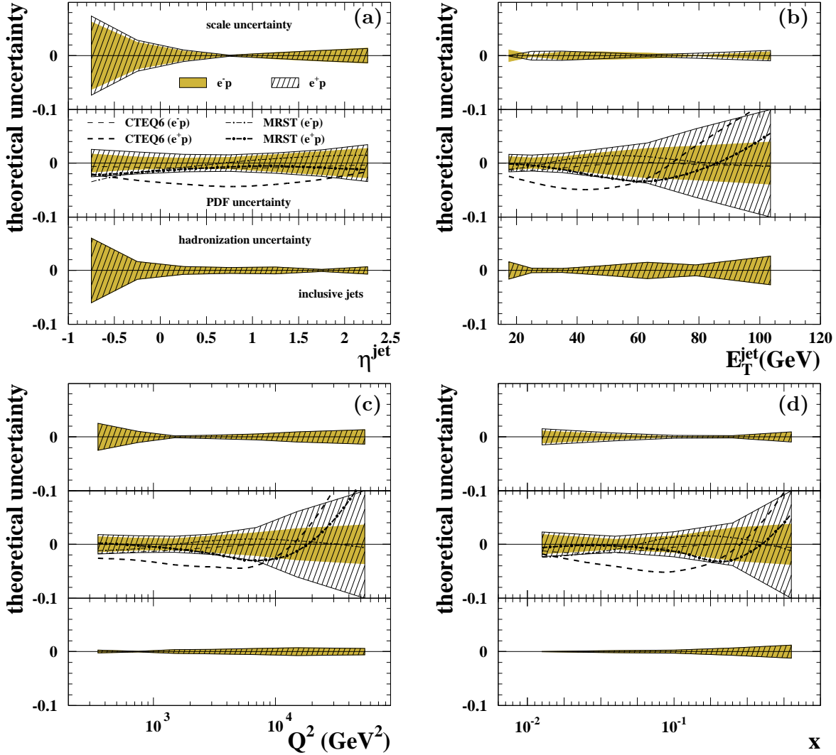
Figure 8.6: Overview of theoretical uncertainties for the inclusive-jet cross sections in CC DIS for jets with E_T^{\text{jet}} > 14 GeV and -1 < \eta^{\text{jet}} < 2.5 in the kinematic regime given by Q^2 > 200 GeV 2 and y < 0.9 as functions of (a) \eta^{\text{jet}} , (b) E_T^{\text{jet}} , (c) Q^2 and (d) x in e^-p (shaded areas) and e^+p (hatched areas) collisions. Shown are the relative uncertainties induced by the variation of the renormalization scale \mu_R , the uncertainties on the proton PDFs and hadronization model. Also shown are the relative differences between the NLO QCD calculations using the CTEQ6 (dashed lines) or MRST (dot-dashed lines) PDF sets to the calculations based on the ZEUS sets.
