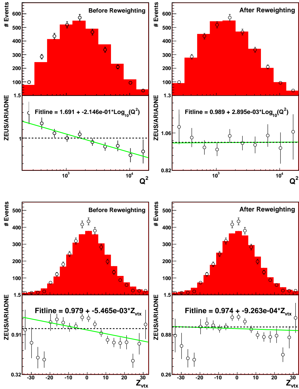
Figure 11.2: Plots comparing detector level distributions of e^+p data versus ARIADNE. All details as in figure 11.1.
