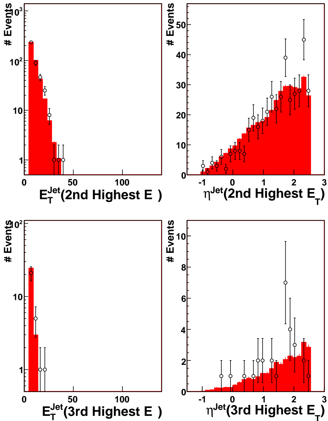
Figure 10.3: Comparison between detector level jet quantities of e^+p data and ARIADNE. All details as in figure 7.2.
