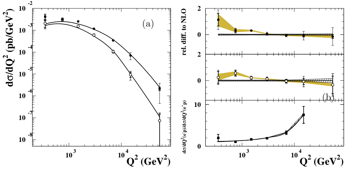
Figure 8.9: Unpolarized e^-p (filled circles) and e^+p (open circles) dijet differential cross sections as a function of Q^2 are shown in (a). The relative difference to NLO pQCD calculations are shown in the upper two portions of (b), while the ratio of e^-p and e^+p cross sections are shown in the bottom portion.
