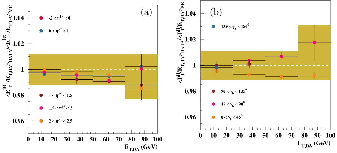
Figure 7.13: E_T reconstruction in bins of \eta^{jet} (a) and \gamma_H (b) vs. E_{T,DA} for e^-p NC DIS ARIADNE, where E_{T,DA} is the transverse energy of the isolated electron. The vertical axis represents the double ratio of ZEUS Data over MC for the quantities E_T^{jet}/E_{T,DA} (a) and P_T^H/E_{T,DA} (b), where P_T^H is the transverse momentum of the entire hadronic system.
