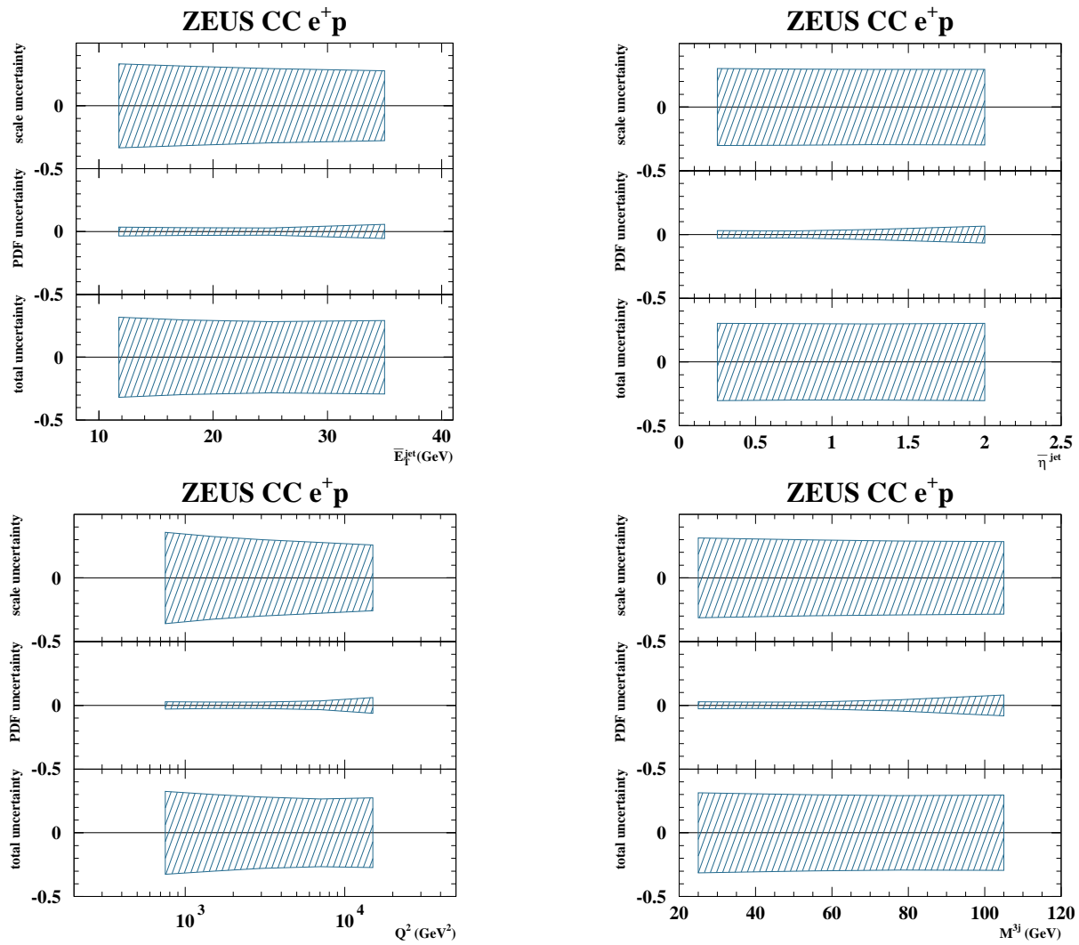
Figure 13.6: Trijet Theoretical Uncertainties e^+p for NLO calculations provided by the MEPJET program.
