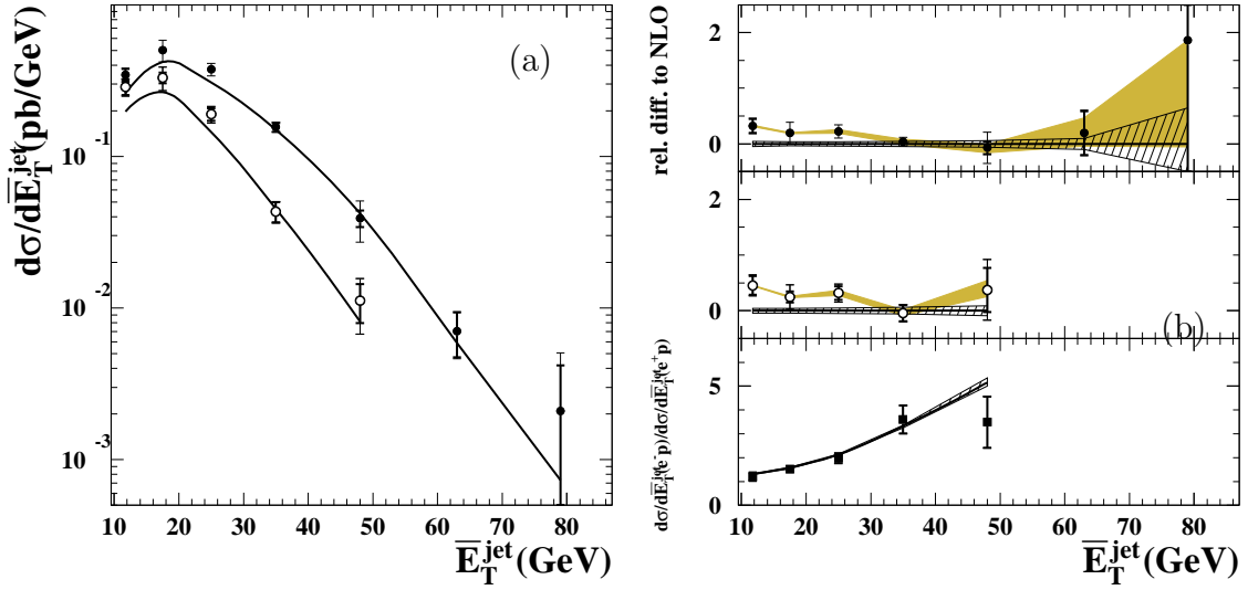
Figure 8.8: Unpolarized e^-p (filled circles) and e^+p (open circles) dijet differential cross sections as a function of \bar{E}_T^{\text{jet}} are shown in (a). The relative difference to NLO pQCD calculations are shown in the upper two portions of (b), while the ratio of e^-p and e^+p cross sections are shown in the bottom portion.
