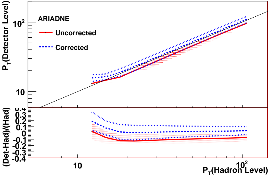
Figure 7.4: Comparison between hadron- and detector-level P_T^{\text{miss}} for e^-p CC DIS ARIADNE. Central lines indicate the mean reconstructed value, while the outer lines and shaded regions indicate \pm 1 -standard-deviations obtained from a Gaussian fit in the reconstructed values for each value of generated P_T^{\text{miss}} .
