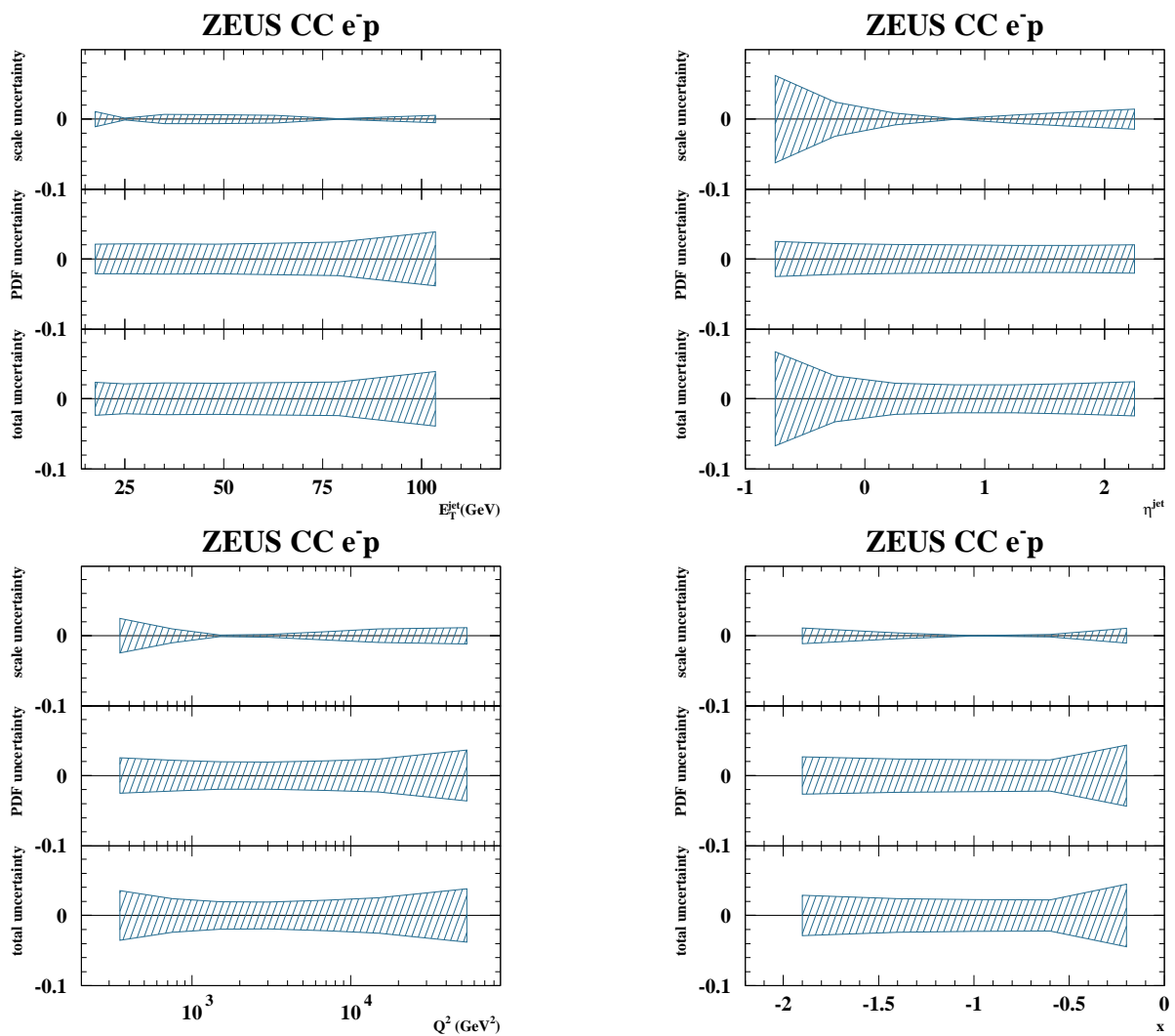
Figure 13.1: Inclusive Jet Theoretical Uncertainties e^-p for NLO calculations provided by the MEPJET program.
