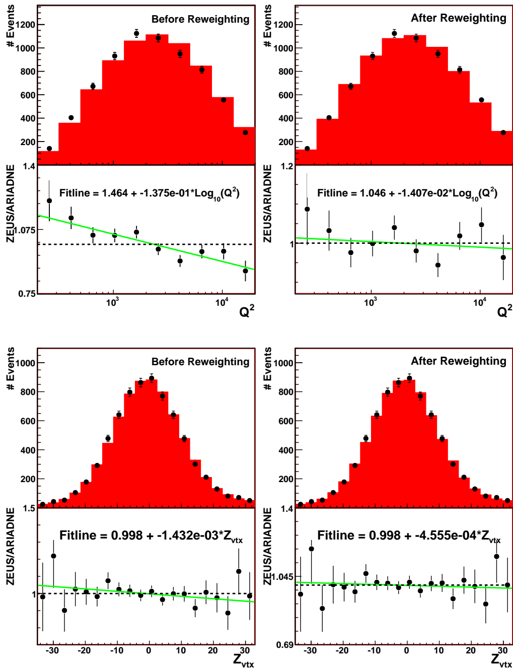
Figure 11.1: Plots comparing detector level distributions of e^-p data versus ARIADNE. The two upper plots show Q^2 , while the bottom two show z_{vtx} . The left two plots show distributions without monte carlo reweighting, while the right two show the same data distributions, but compared to reweighted monte carlo. The monte carlo distributions have been area-normalized to the data. Below each distribution, a ratio plot is shown of data/ARIADNE. A linear \chi^2 fit is shown for each ratio.
