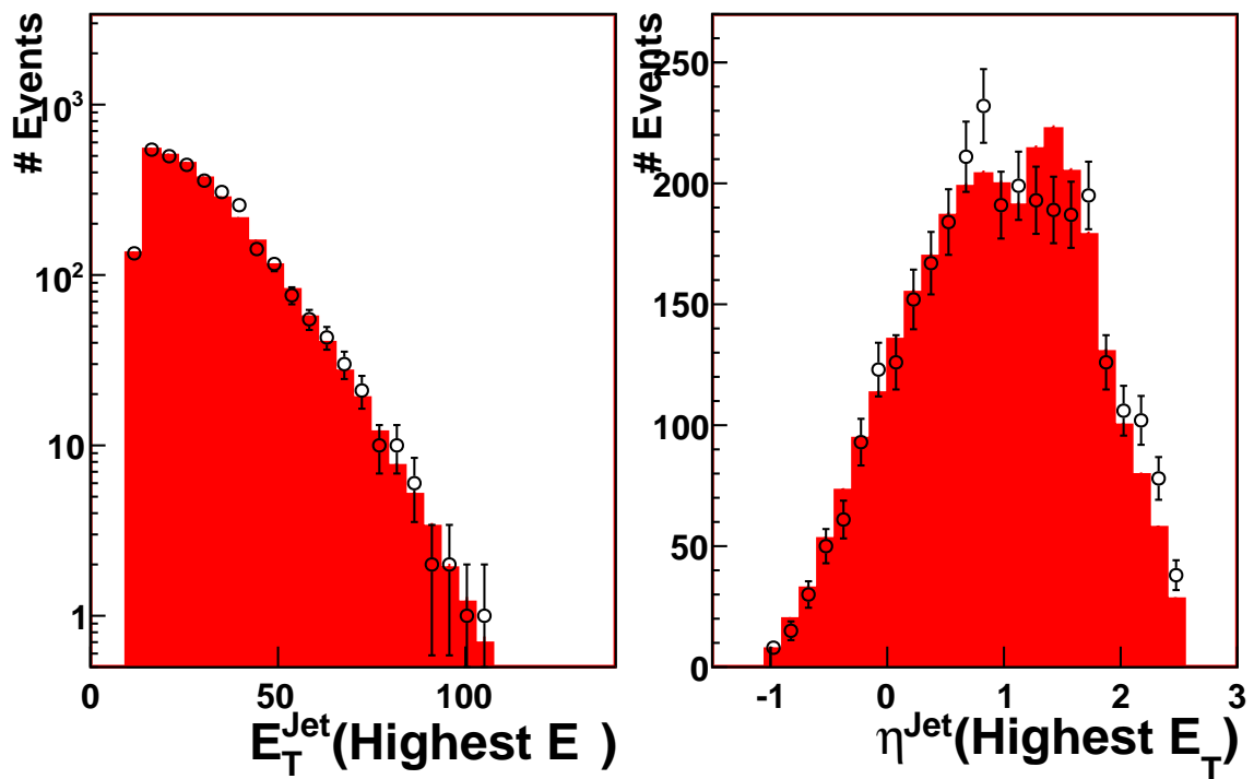
Figure 10.2: Comparison between detector level jet quantities of e^+p data and ARIADNE. All details as in figure 7.2.
