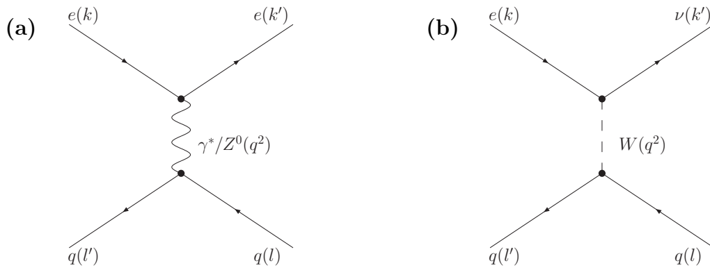
Figure 1.2: L.O. Feynman Diagrams for NC and CC DIS
