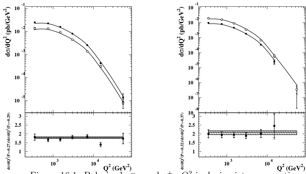
Figure 16.1: Polarized e^-p and e^+p Q^2 inclusive-jet cross sections
