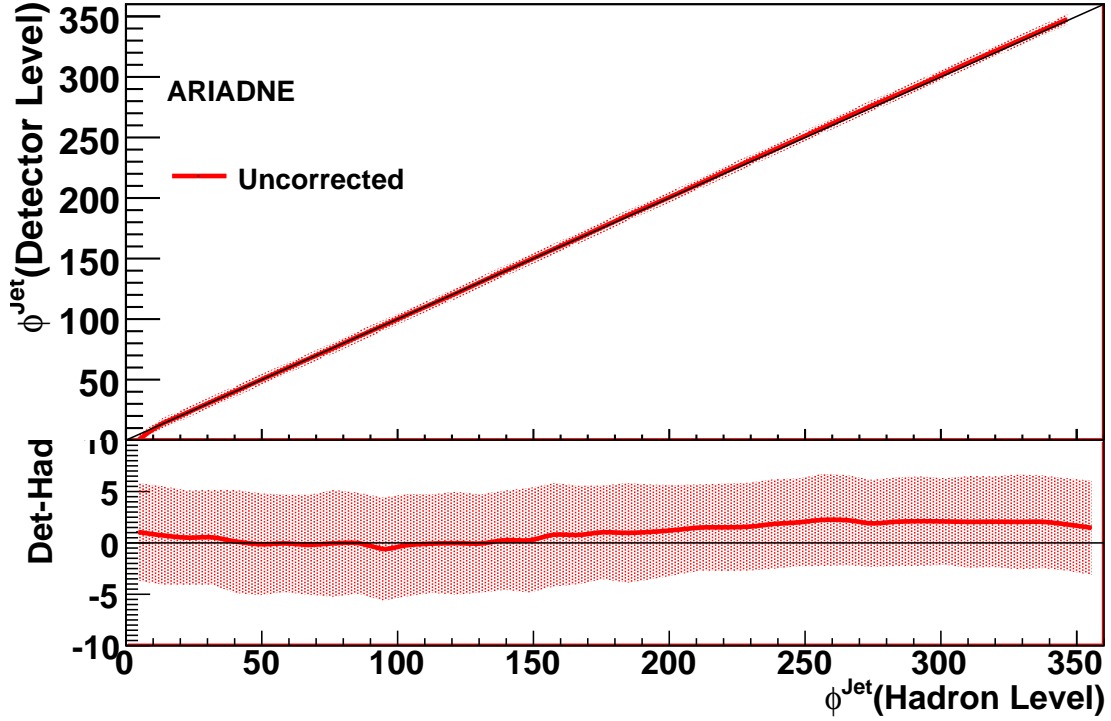
Figure 7.10: Comparison between hadron- and detector-level \phi^{\text{jet}} for e^-p Cc DIS ARIADNE. Central lines indicate the mean reconstructed value, while the shaded region indicates \pm 1 -standard-deviations obtained from a Gaussian fit in the reconstructed values for each value of generated \phi^{\text{jet}} .
