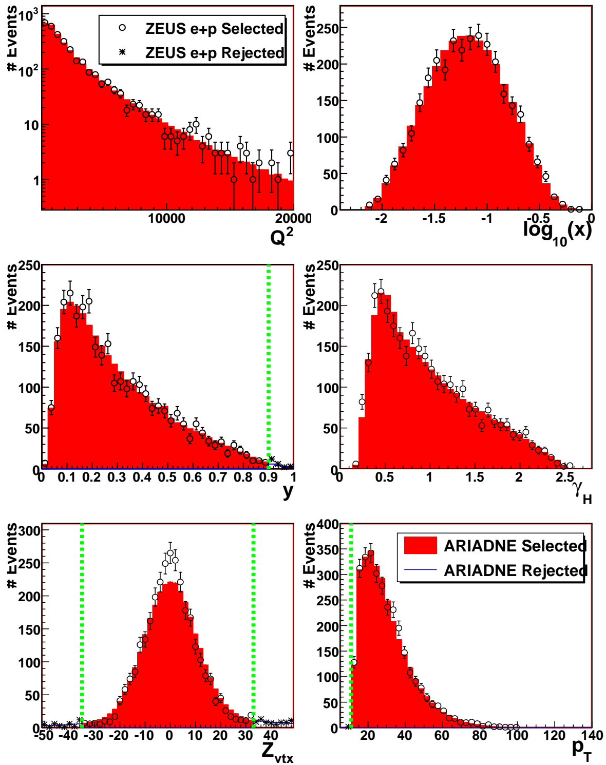
Figure 10.1: Comparison between detector level kinematic quantities of e^+p data and ARIADNE. All details as in figure 7.1.
