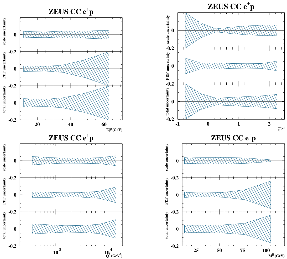
Figure 13.5: Di-jet Theoretical Uncertainties e^+p for NLO calculations provided by the MEPJET program.
