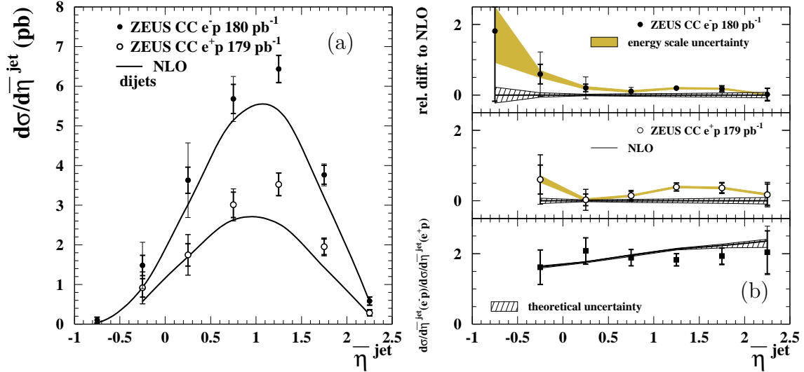
Figure 8.7: Unpolarized e^-p (filled circles) and e^+p (open circles) dijet differential cross sections as a function of \bar{\eta}^{\text{jets}} are shown in (a). The relative difference to NLO pQCD calculations are shown in the upper two portions of (b), while the ratio of e^-p and e^+p cross sections are shown in the bottom portion.
