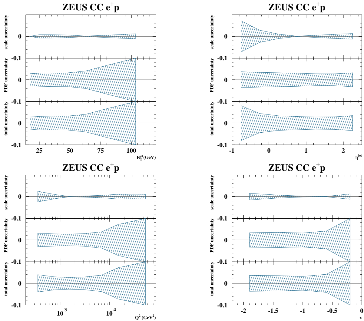
Figure 13.4: Inclusive Jet Theoretical Uncertainties e^+p for NLO calculations provided by the MEPJET program.
