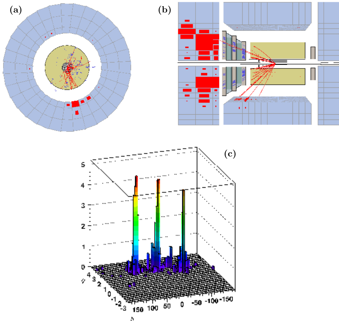
Figure 8.11: Three-jet candidate event in CC DIS in the ZEUS detector. The event is viewed in the x - y plane in (a), the z - r view in (b), and E_T of CAL deposition \eta - \phi plane in (c). In (a) and (b), reconstructed tracks are superimposed over CTD hits, and CAL depositions are drawn proportional to the energy deposited. In (a), only the energy deposition in the barrel calorimeter is shown. In (a) an imbalance in the azimuthal distribution of tracks is observed. In (c), three broad CAL depositions are observed, which are separated in the \eta - \phi plane. In (b), these are observed to penetrate into the second hadronic section of the CAL. These depositions were reconstructed as three jets.
