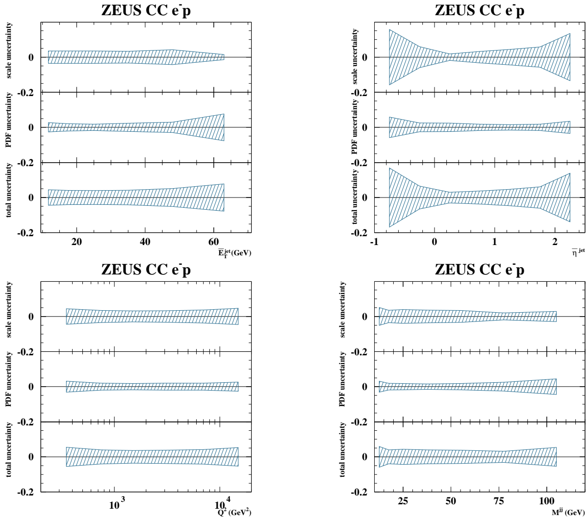
Figure 13.2: Dijet Theoretical Uncertainties e^-p for NLO calculations provided by the MEPJET program.
