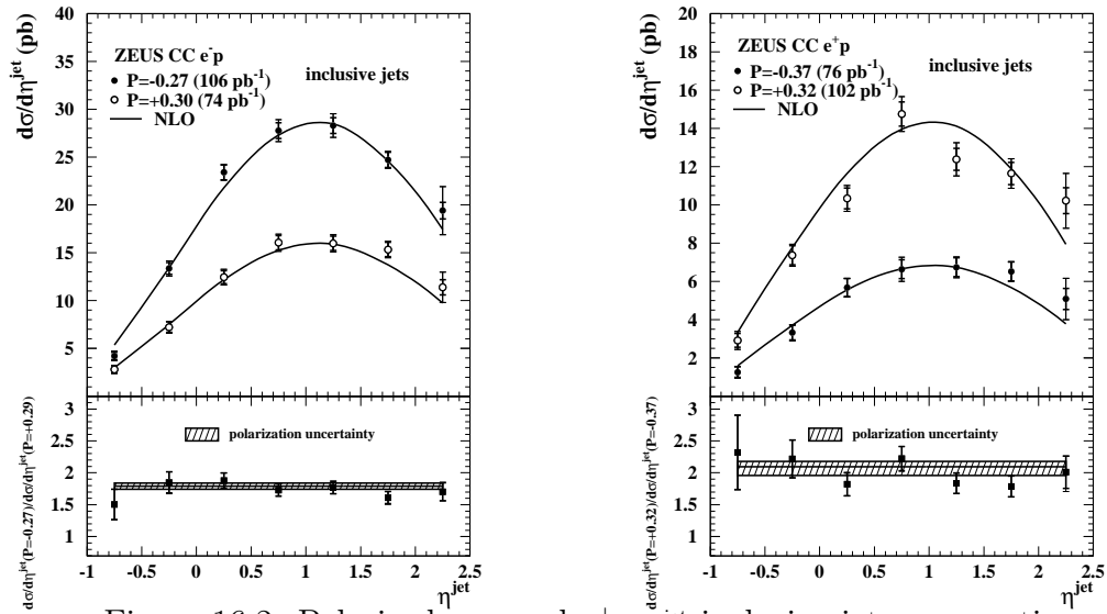
Figure 16.2: Polarized e^-p and e^+p \eta^{\text{jet}} inclusive-jet cross sections
