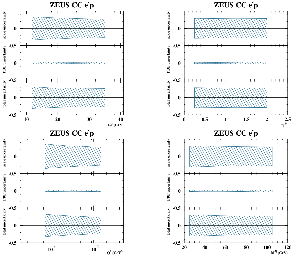
Figure 13.3: Trijet Theoretical Uncertainties e^-p for NLO calculations provided by the MEPJET program.
