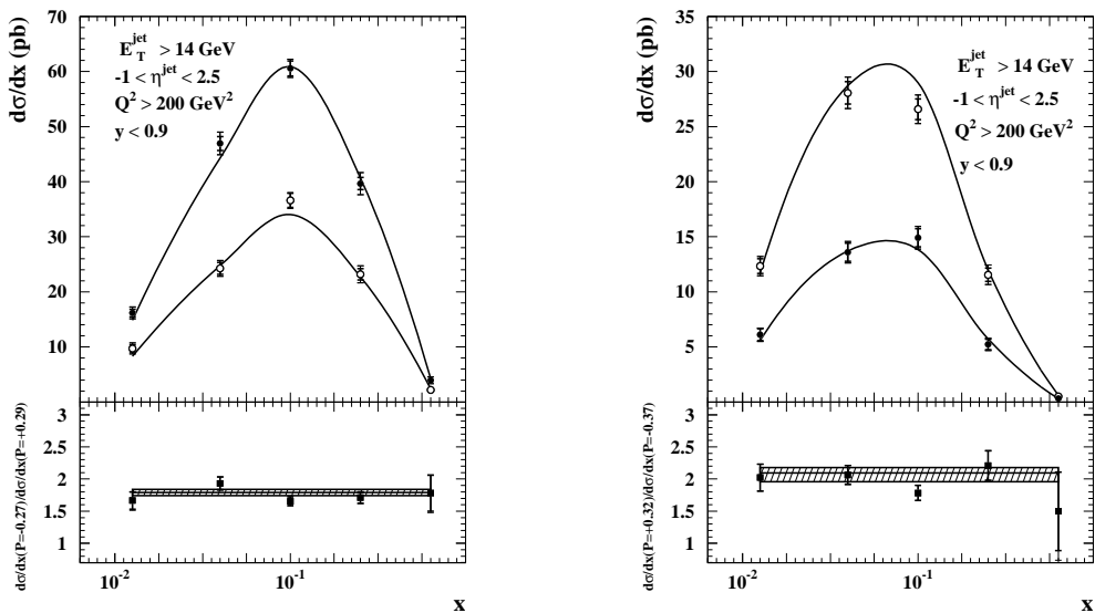
Figure 16.3: Polarized e^-p and e^+p x inclusive-jet cross sections
